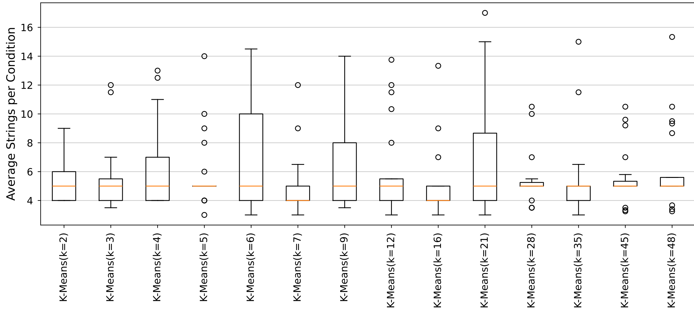
YARA Rules Average Strings per Condition Distribution (Cluster4_Size48 dataset)
